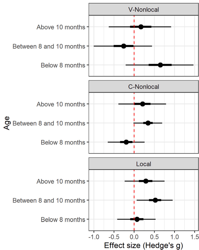
Fig. 6. Effect size by binned Age crossed with Dependency Type, with the point representing the median, and the thicker and thinner intervals encompassing the central 50% and 95% Credible Intervals for values of effect size, respectively. The dashed vertical line marks an effect size of zero.
