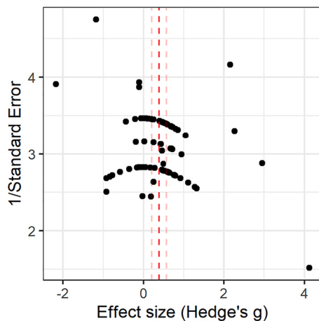
Fig. 3. Funnel plot which graphs 1/Standard Error (vertical axis) as a function of Hedge's g (on the horizontal axis). Dotted lines indicate median meta-analytic effect size from model reported in Section 3.1, with paler lines delimiting the 95% Credible Interval.
